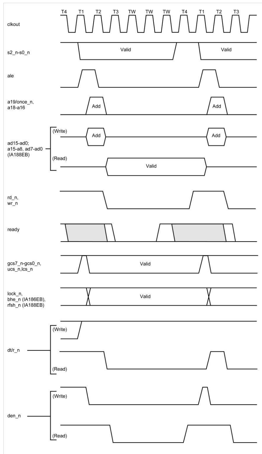
Figure 28. Ready Timing
