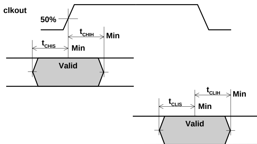
Figure 12. AC Input Characteristics
